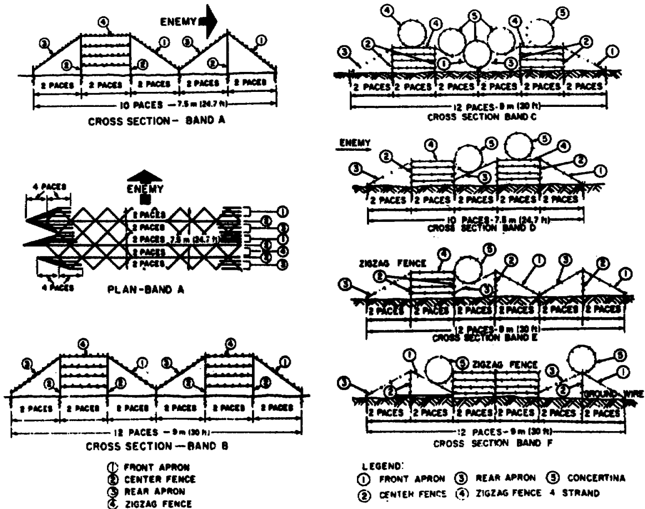
Figure 4-35. Combination bands of wire obstacles.
